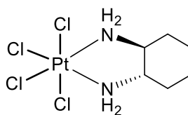
Ormaplatin
