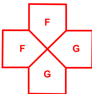
cis - F_2G_2
