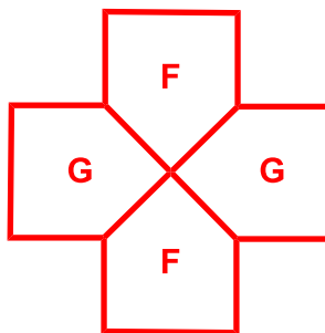
trans - F_2G_2
