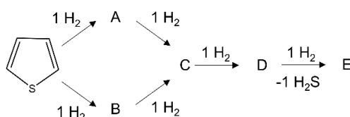
Figure 1. Thiophene hydrodesulfurization process.
